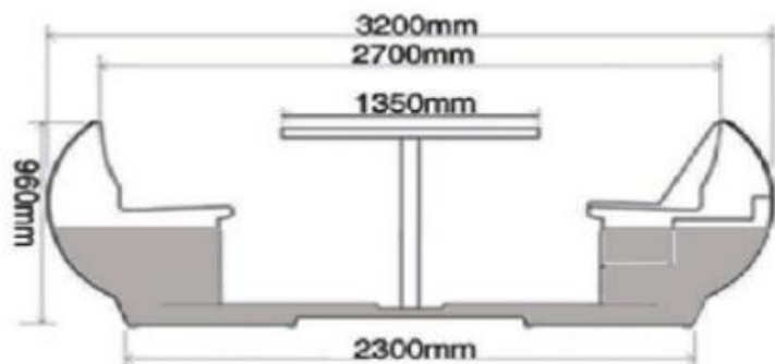
游艇内部聚氨酯发泡填充 Puf foam padding inside the boat
